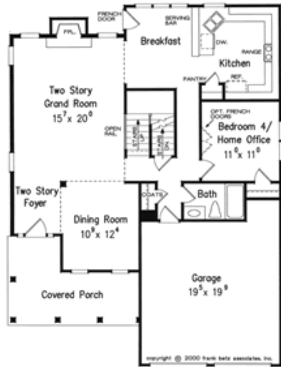
Floor 1
