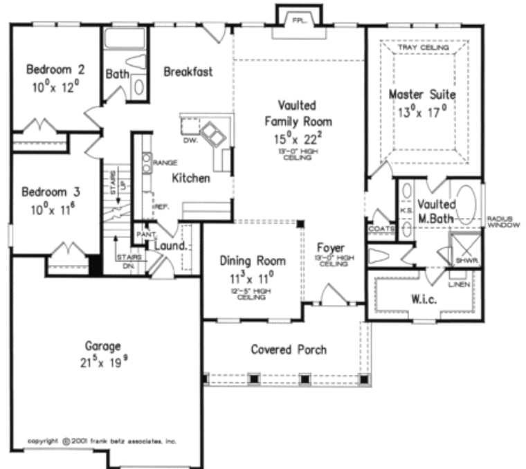
Floor 1
