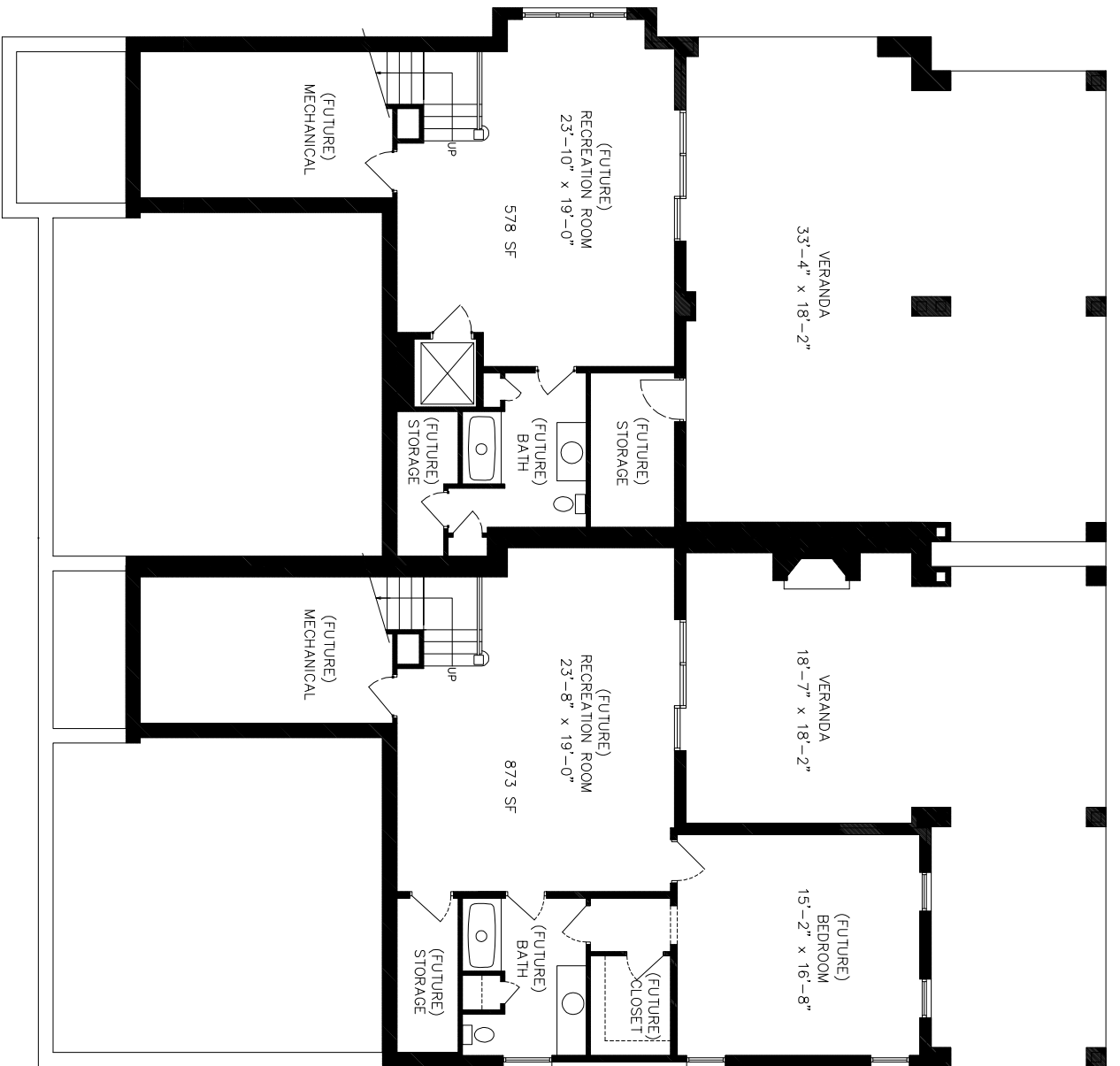
BASEMENT PLAN
